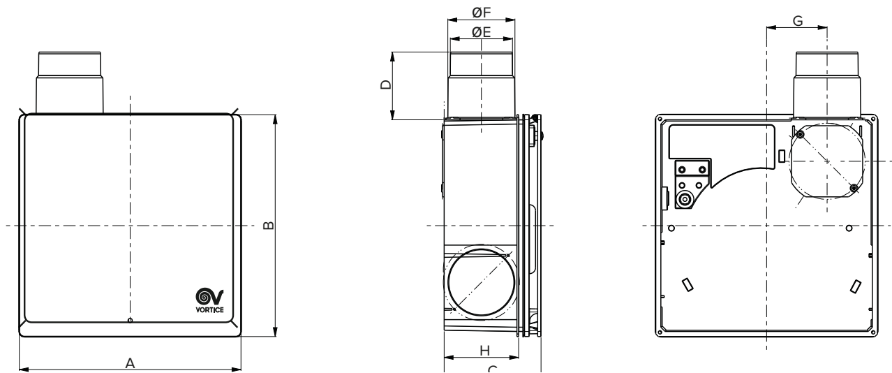
RECESSED VERSION
